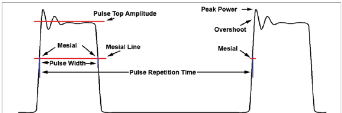
Figure 1 • Pulse Waveform Detail.
