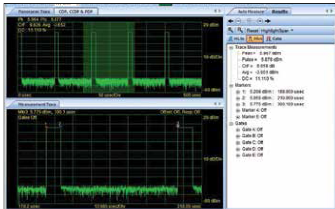
Figure 3 • Pulse Profile Measurement.
